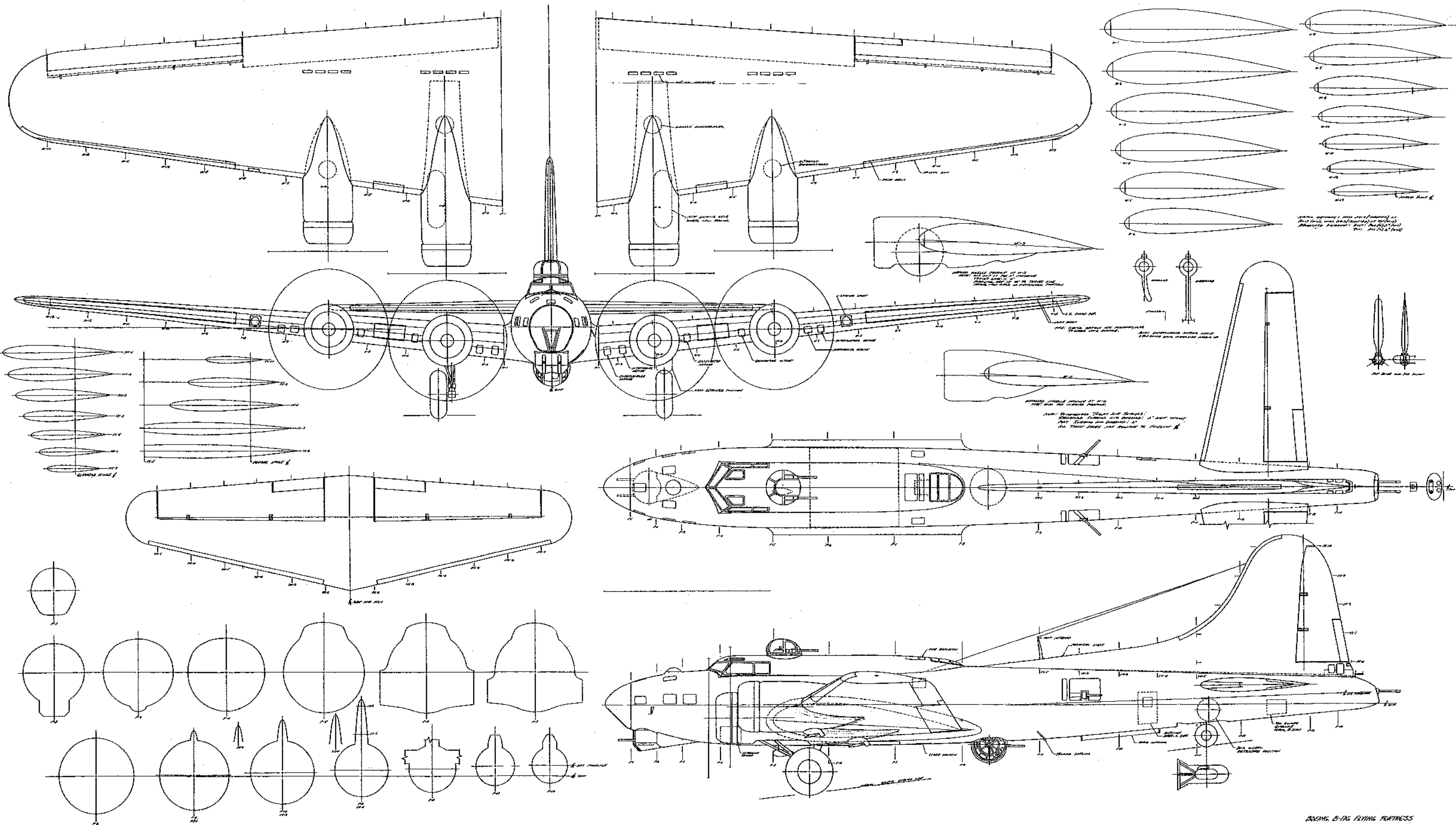
BOEING B-17G FLYING FORTRESS
